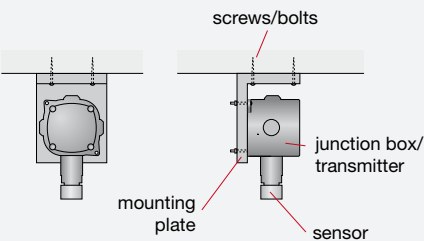
CEILING MOUNTED
