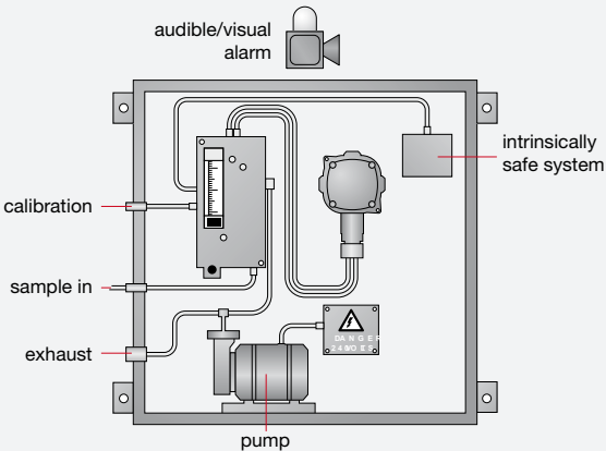
TYPICAL SAMPLING/ASPIRATING SYSTEM
