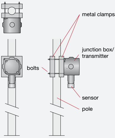
POLE MOUNTED
